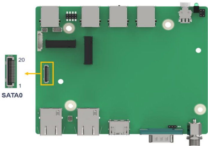
Figure 4-10: SATA 6Gb/s Drive Connectors Location
