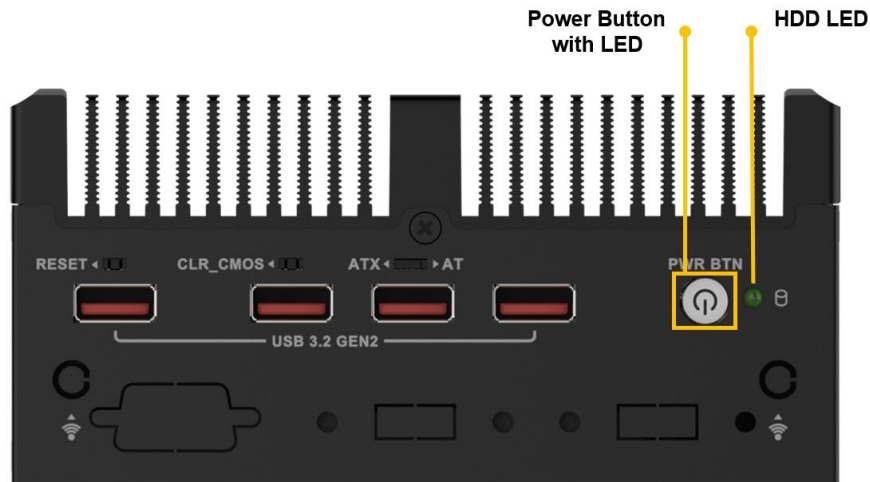
Figure 3-21: Power Button & LED
