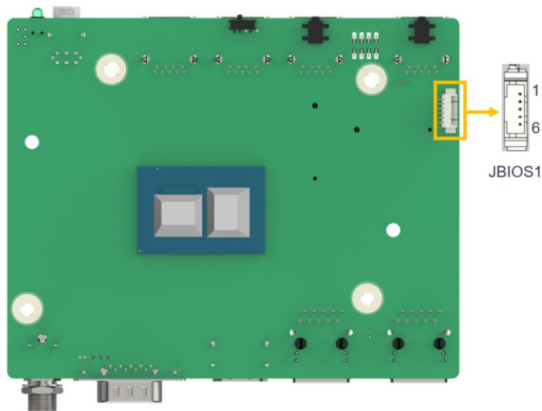
Figure 4-11: Flash SPI ROM Connector Location
