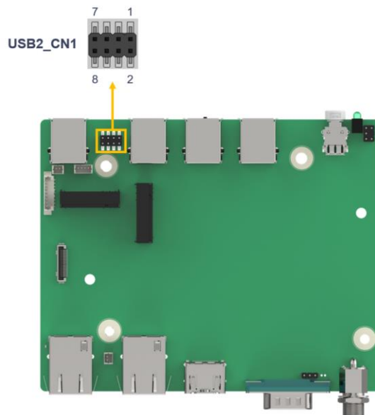
Figure 4-14: Internal USB 2.0 Connectors Locations
