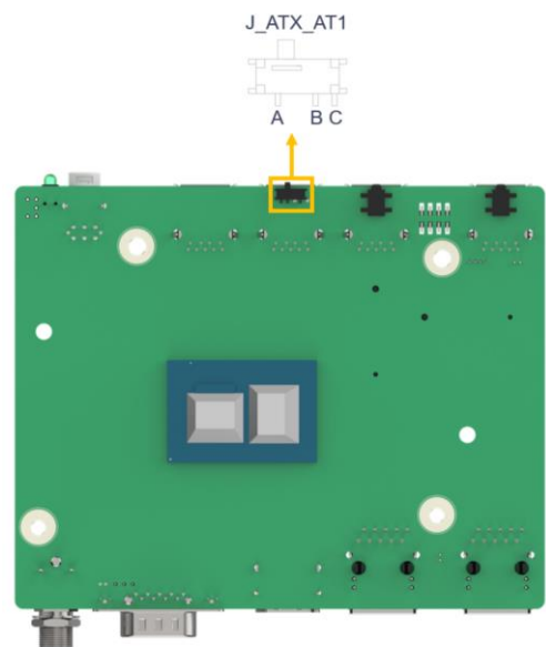
Figure 4-3: AT/ATX Power Mode Switch Locations
