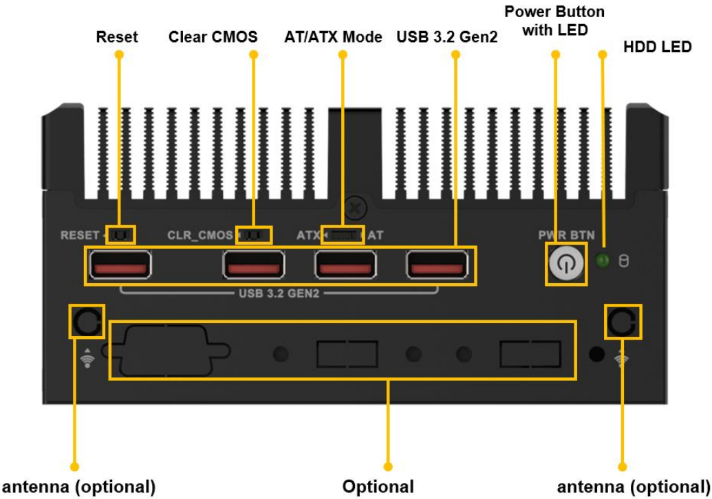
Figure 1-2: Front Panel
