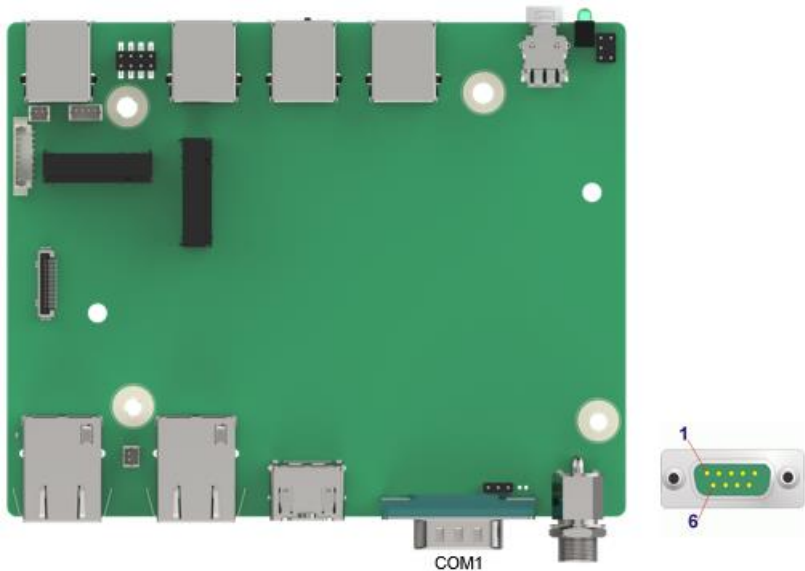
Figure 4-8: RS-232/422/485 Serial Port Connector Location
