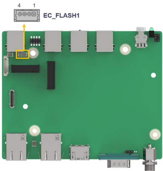
Figure 4-12: Flash EC ROM Connector Location
