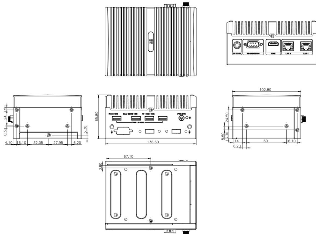
Figure 1-4: Physical Dimensions
