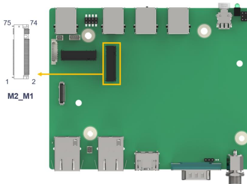
Figure 4-16: M.2 M-key Slot Location
