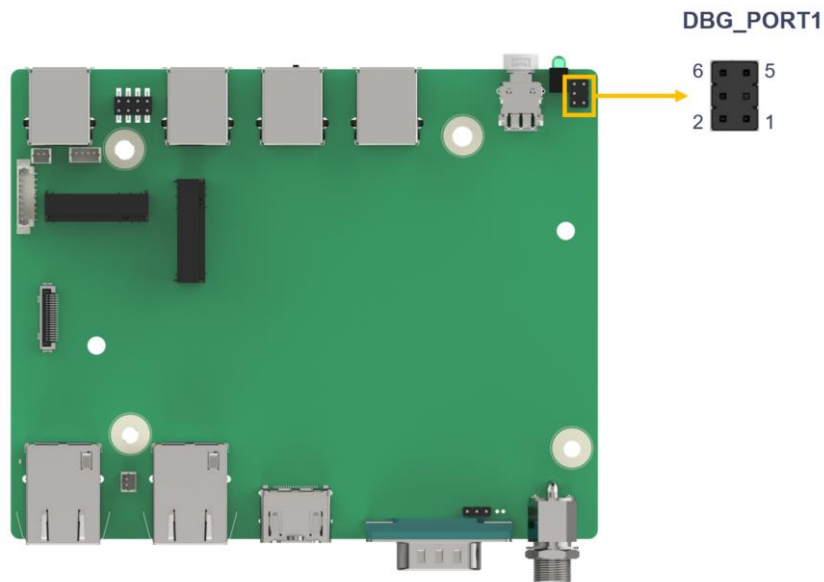
Figure 4-13: EC Debug Connector Location
